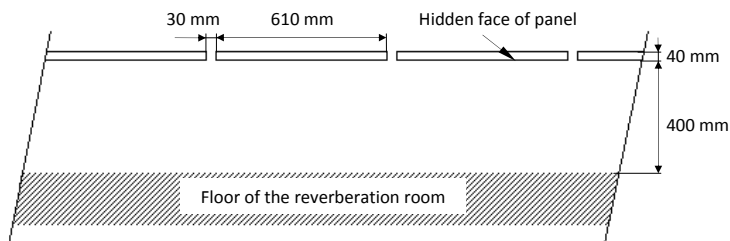
Arrangement of the test specimen (B2019-54-M607)
