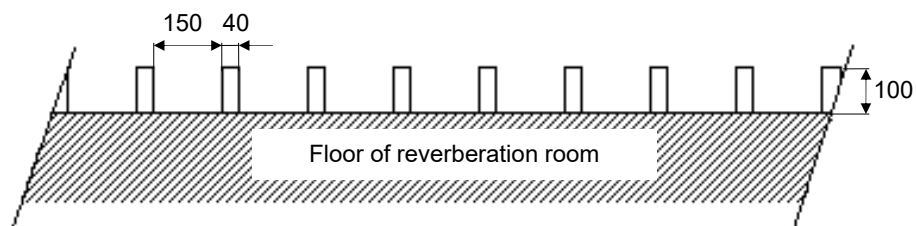
Arrangement of the test specimen (B2023-195-M952). Cotes in mm
