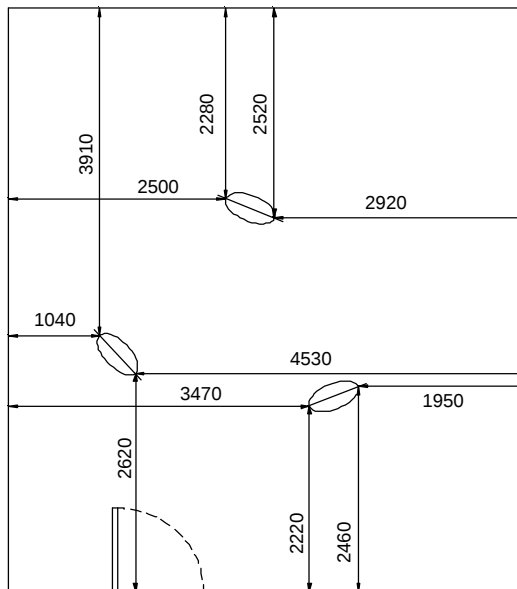
Arrangement of the test specimen (B2019-83-M658)
