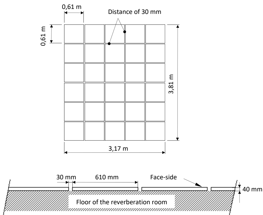
Arrangement of the test specimen (B2021-146-M841)
