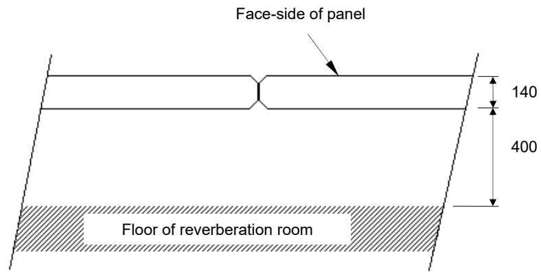
Arrangement of test specimen (110259-7). Cotes in mm
